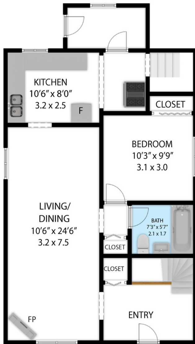
MAIN FLOOR 76 SQ.M - 825 SQ.FT
