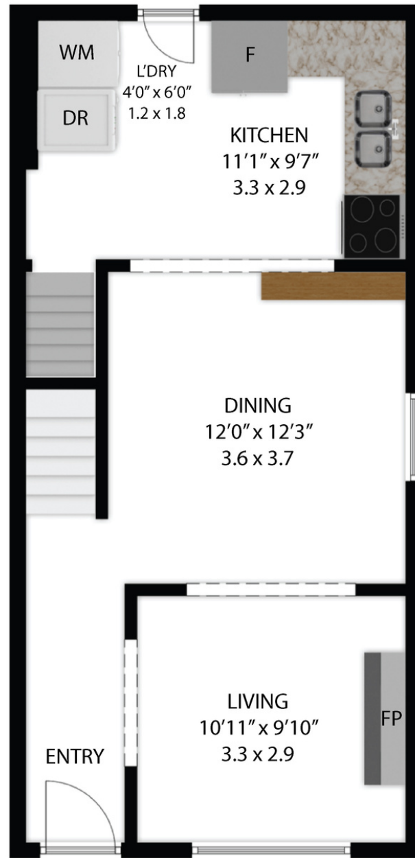
MAIN FLOOR
