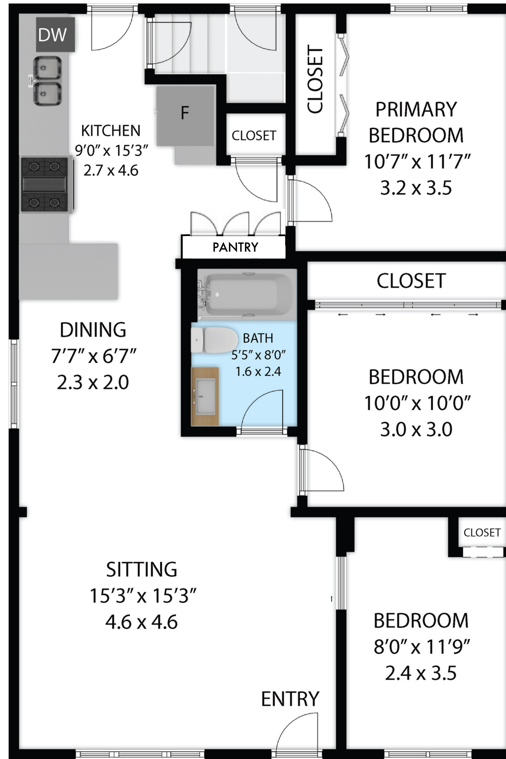
MAIN FLOOR
