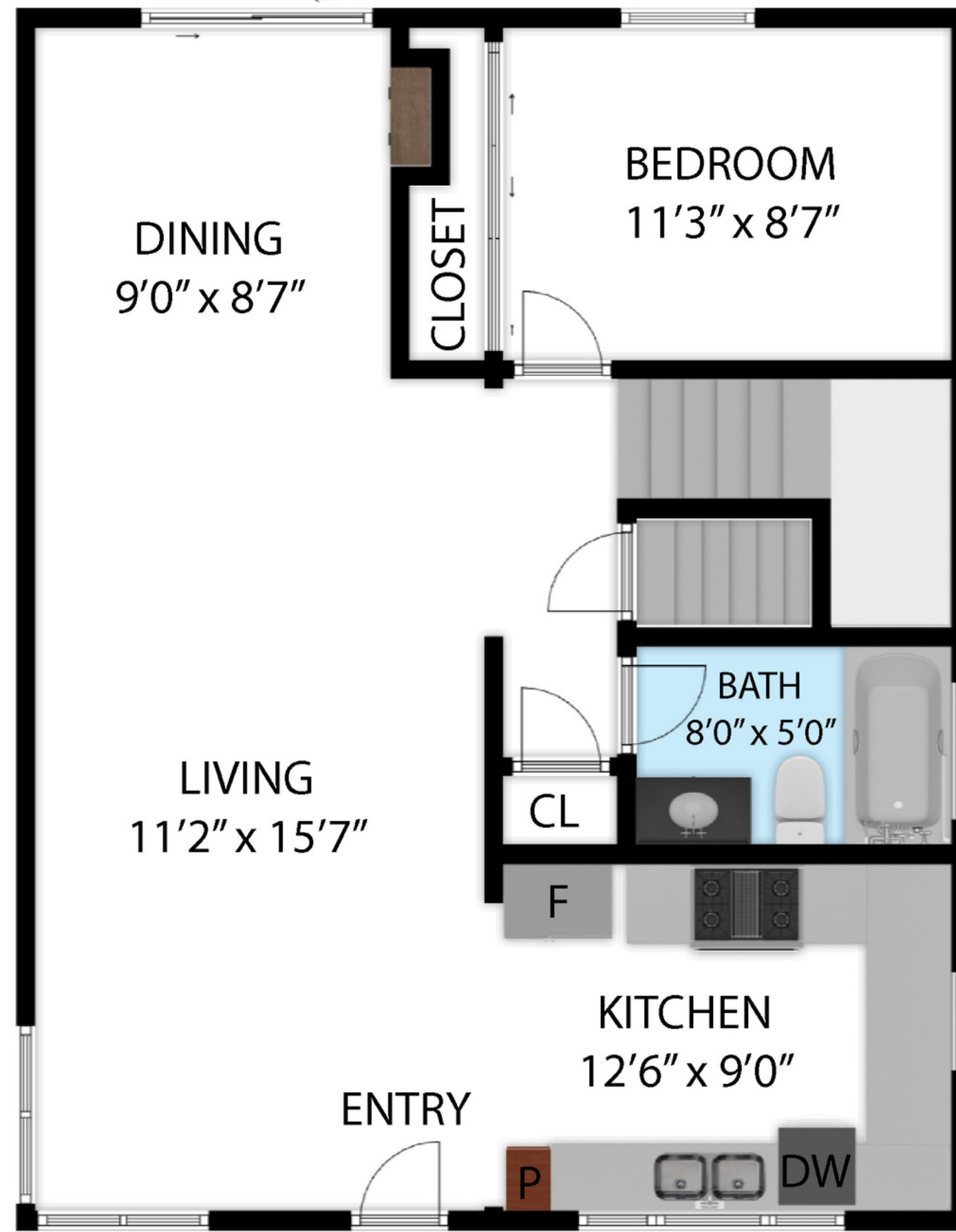
MAIN FLOOR
