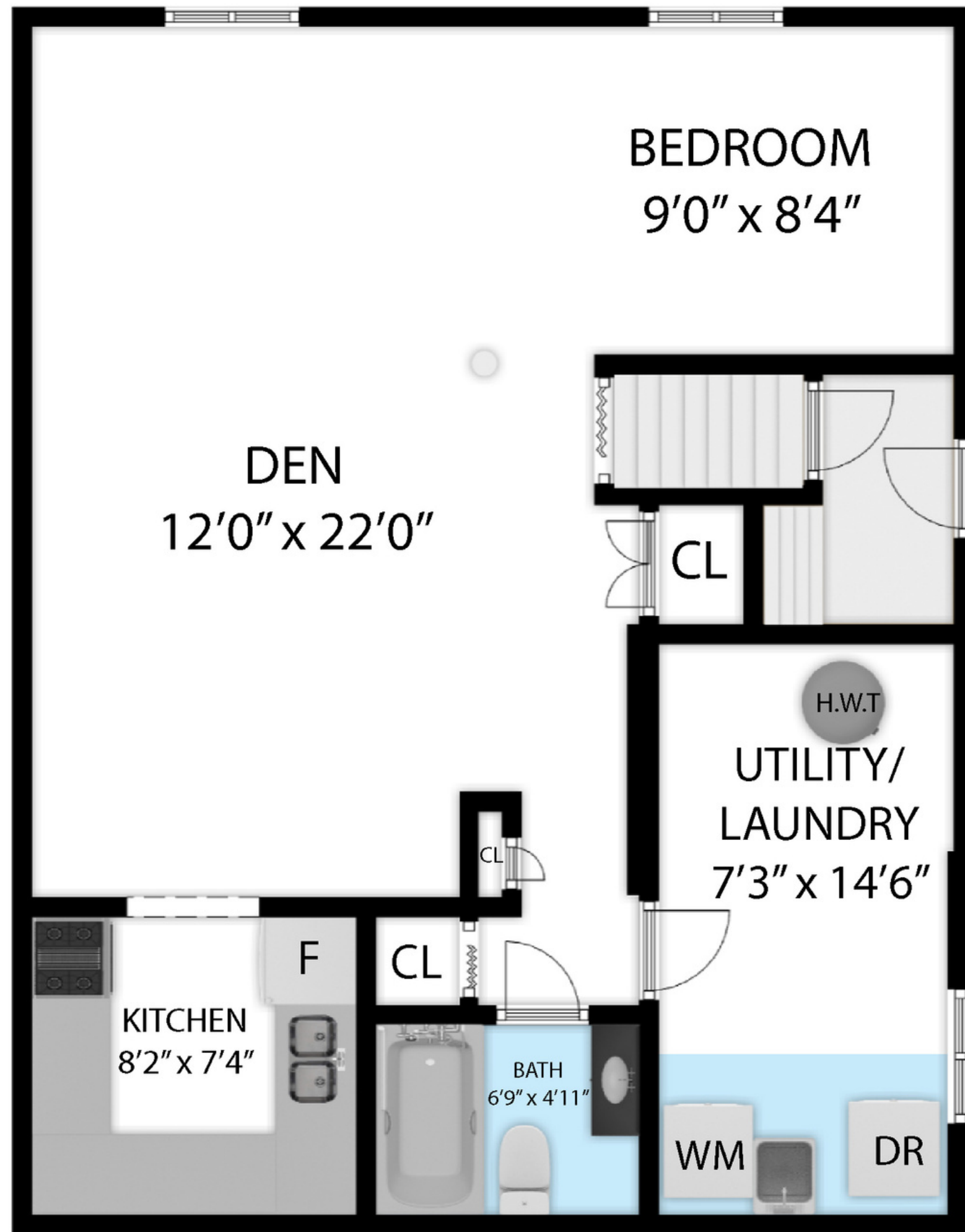
BASEMENT
