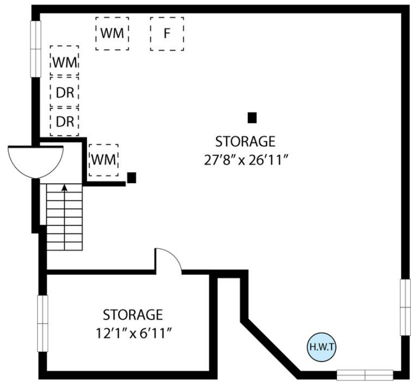
BASEMENT
